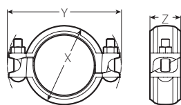
STYLE 607 JOINT ASSEMBLED
