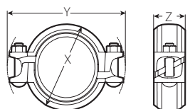
STYLE 607 PRE-ASSEMBLED (INSTALLATION-READY CONDITION)
